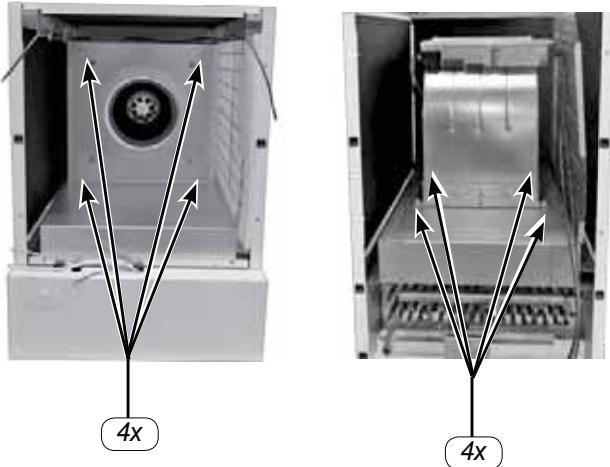
Ventilator Elan 10/16 2.0
